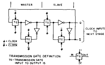
Fig. 11— Basic frequency-dividing stage.
