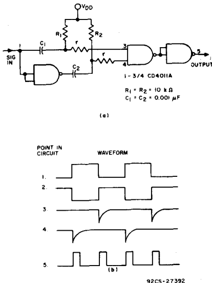
Fig. 23 - (a) Frequency-doubler schematic, (b) waveforms.
