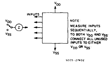
Fig. 16 - Input current.
