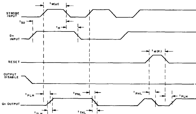
Fig. 12 — Test waveforms.
