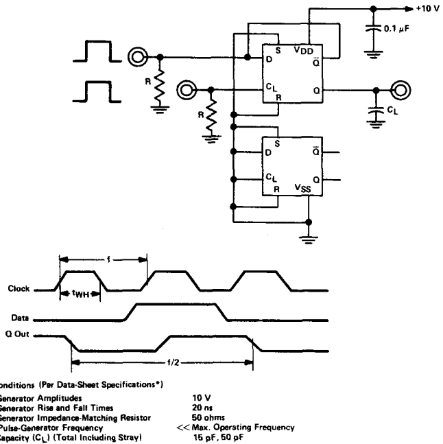
92CS-28383 Fig. 27 - Test circuit for measuring minimum clock-pulse width in a CD4013A/B.
