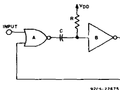
Fig. 11 - CMOS monostable circuit. 92CS-22675
