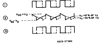
Fig. 8 - Waveforms showing effects of transfer voltage on multivibrator frequency.
