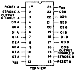
TERMINAL ASSIGNMENT
