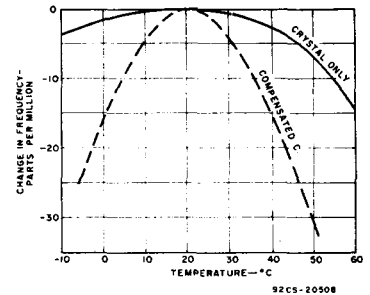
Fig. 7— Effect of temperature on crystal frequency.
