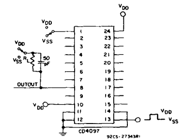
Fig. 12—Turn-on and turn-off propagation delay—inhibit input to signal output (e.g. measured on channel 1).
