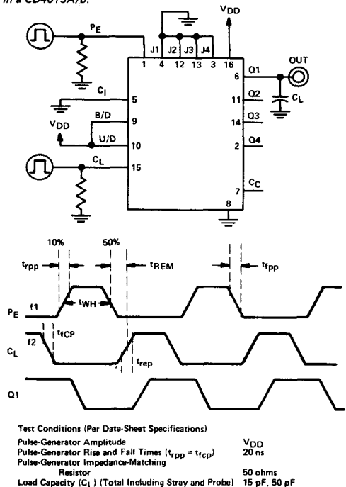
92CS-28382 Fig. 29 - Test circuit for measuring preset-enable removal time in a CD4029A/B.
