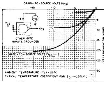
Fig. 2b - Typical p-channel characteristics.
