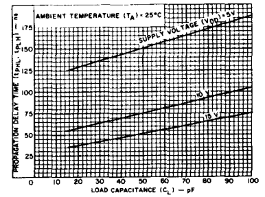
Fig. 7 — Typical propagation delay time vs. load capacitance—data to \bar{Q} .
