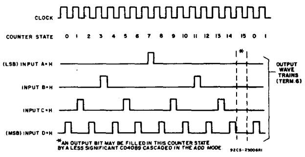
Fig. 15 - Timing diagram.
