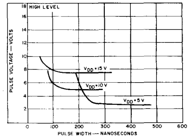
Fig. 5 - Voltage noise immunity of the CD4093B.
