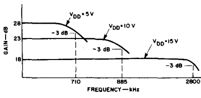
(b) TYPICAL CD4001UB LINEAR GAIN
