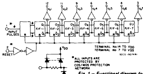
Fig. 1 - Functional diagram for CD4024AD, AE, AF.
