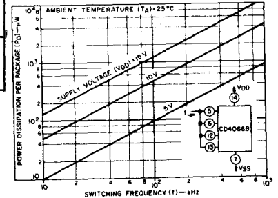
Fig. 9—Power dissipation per package vs. switching frequency.
