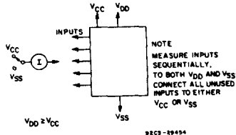
Fig. 15 - Input current.
