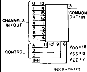
Single 8-Channel Analog Multiplexer/Demultiplexer CD4051B (Page 206)
