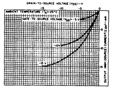
Fig. 4 - Minimum output high (source) current characteristics.
