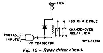
Fig. 10 - Relay driver circuit.
