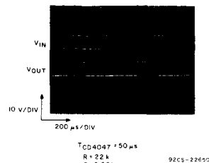
Fig. 29 - Low-pass-circuit waveforms.
