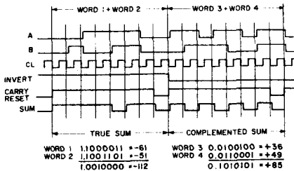
Fig. 4 - CD4038B timing diagram.
