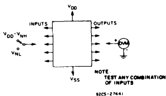
Fig. 15 — Noise-immunity test circuit.
