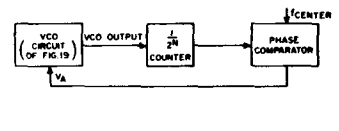
Fig. 21 - VCO used in phase-locked loop.
