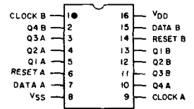
TERMINAL DIAGRAM
