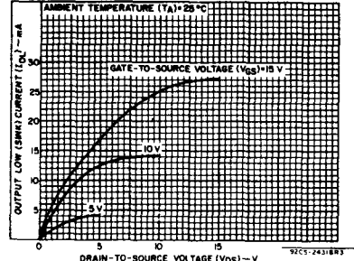
Fig. 3 - Typical output low (sink) current characteristics.
