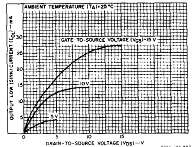
Fig. 3 - Typical n-channel output low (sink) current characteristics.
