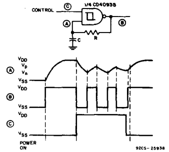
Fig. 18 - Gated astable oscillator.
