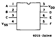
Fig. 2 - Pin assignments of the CD40107BE.
