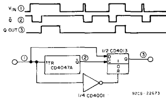
Fig. 23 - Noise-discriminator circuit.
