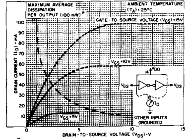
Fig. 2 - Typical output n-channel drain characteristics - true output.
