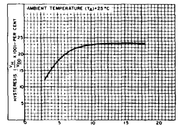
Fig. 13 - Typical per cent hysteresis vs. supply voltage.
