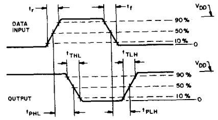
Fig. 14 - Dynamic waveforms.
