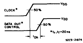
Fig. 7 - Data hold time.
