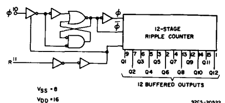
Fig.4 — Functional diagram.
