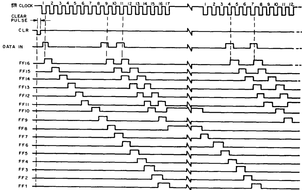
Fig. 4 - Functional timing diagram-shift registers function.
