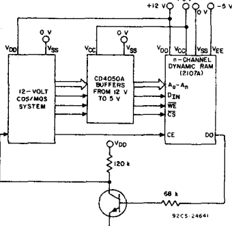
Fig. 10—COS/MOS to n-channel dynamic RAM interface.
