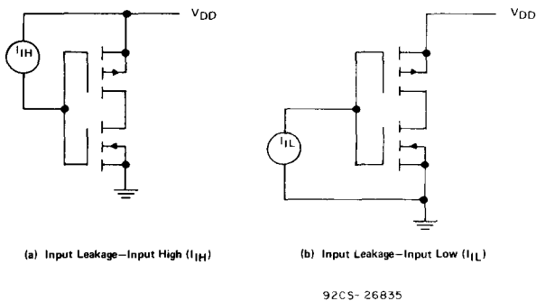
Fig. 9 — Measurement of input leakage.
