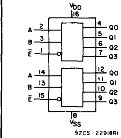
Dual Binary-to-1-of-4 Decoder/Demultiplexer Output "High" on Select
