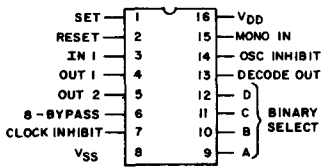
Terminal Assignment
