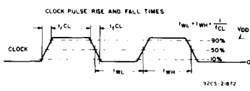
Fig. 5 - Clock pulse rise and fall times.
