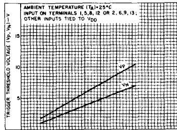
Fig. 12 - Typical trigger threshold voltage vs. V_{DD} .
