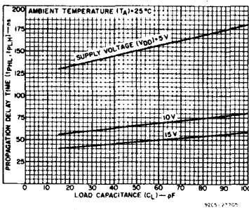
Fig. 7 — Typical propagation delay time vs. load capacitance—SET, RESET to Q, Q.
