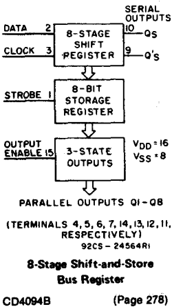
8-Stage Shift-and-Store Bus Register CD4094B (Page 278)
