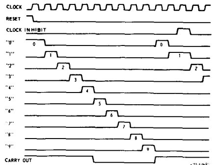
Fig. 2 - Timing diagram.
