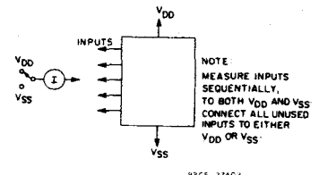
Fig. 16 - Input current test circuit.
