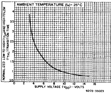
Fig. 14—Variation of low-to-high ( t_{TLH} ) and high-to-low ( t_{TLH} ) transition time with supply voltage.
