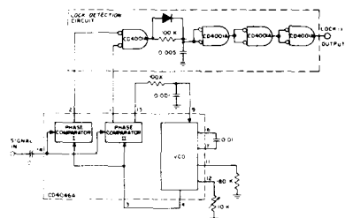
Fig. 15— Lock-detection circuit.
