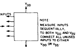
Fig. 12 - Input-current test circuit.
