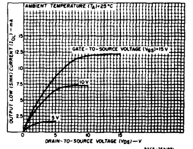
Fig. 2 - Minimum output low (sink) current characteristics.
