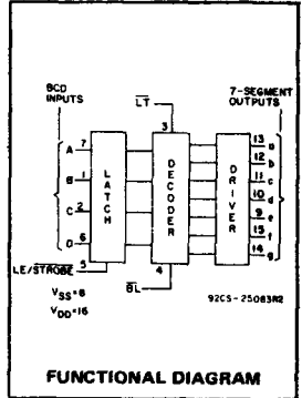
FUNCTIONAL DIAGRAM
