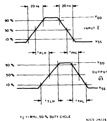
Fig. 18 - CD4555B E-bar input to Q3 output dynamic signal waveforms.
