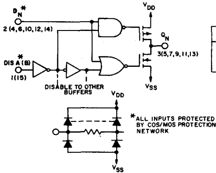
Fig. 1—Logic diagram of 1 to 6 identical buffers.
