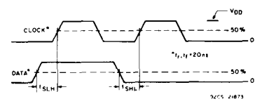
Fig. 6 - Data setup time.
