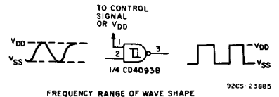
Fig. 16 - Wave shaper.
