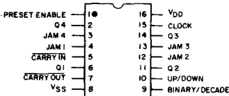
CD4029B Terminal Diagram
