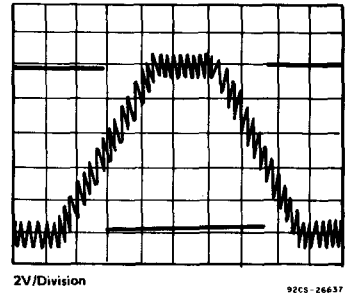
Fig. 19 - Rejection of noise on slow input edge.
