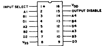
TERMINAL ASSIGNMENT
