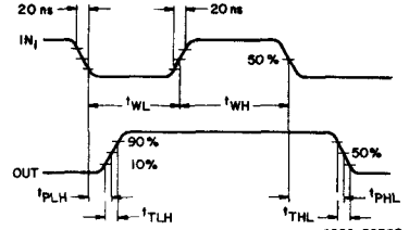
Fig. 22—Input waveforms for switching-time test circuit.
