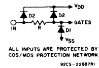
Fig. 1 - Functional diagrams.
