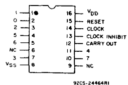
TOP VIEW CD4022B TERMINAL DIAGRAM
