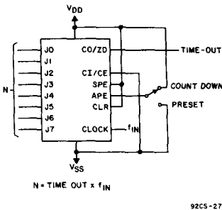
Fig. 19 - Programmable timer.
