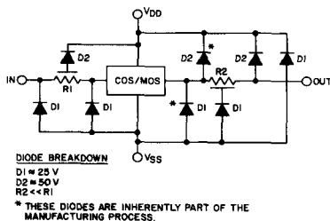
Fig. 2 - Improved protection network.
