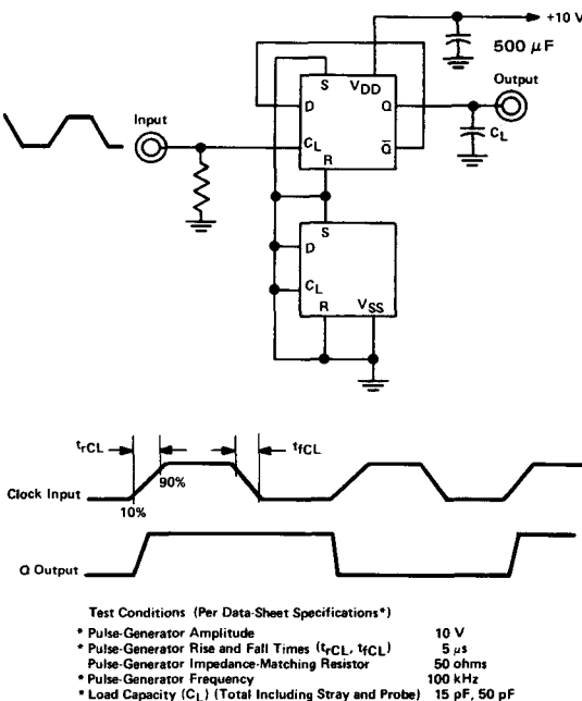
92CS-28381R Fig. 28 - Test circuit for measuring maximum clock-rise and fall time in a CD4013A/B.
