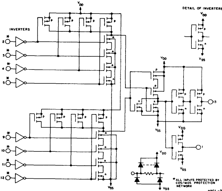
Fig. 8 - Schematic diagram.
