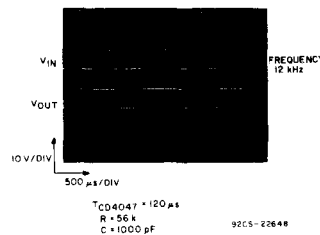
Fig. 33 - Envelope-detector-circuit waveforms.
