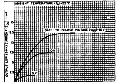
Fig. 4—Minimum output low (sink) current characteristics.
