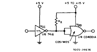
Fig. 4—TTL to COS/MOS at a V DD greater than 5 volts.
