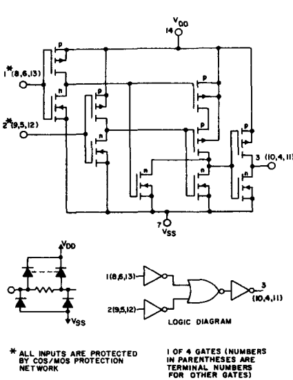
Fig. 7 - Schematic and logic diagrams for CD4011B.
