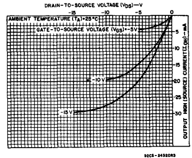
Fig. 10 - Typical output high (source) current characteristics.
