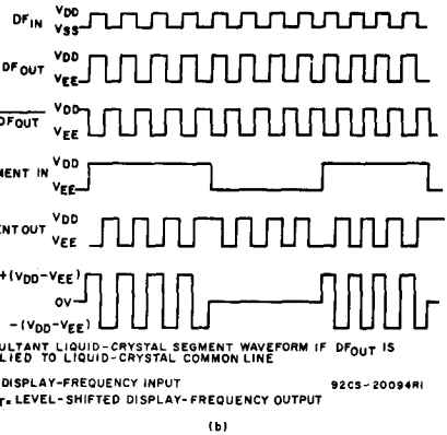
Fig. 17 - Display-driver circuit for one segment line and waveforms.
