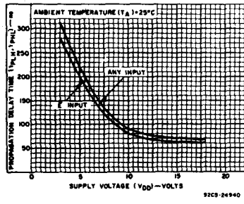
Fig. 9 - Typical propagation delay time vs. supply voltage.
