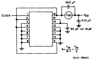
Fig. 17 - Dynamic power dissipation test circuit ( f \geq 2 mode).
