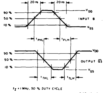
Fig. 16 - CD4555B B input to Q3 output dynamic signal waveforms.
