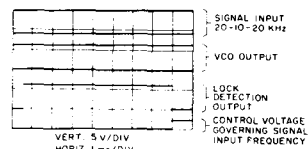
Fig. 16— Lock-detection-circuit waveforms.
