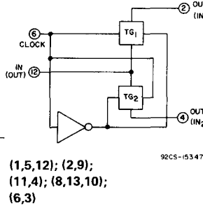
Fig. 2 - Sample COS/MOS logic circuit arrangements using type CD4007UB (Cont'd).
