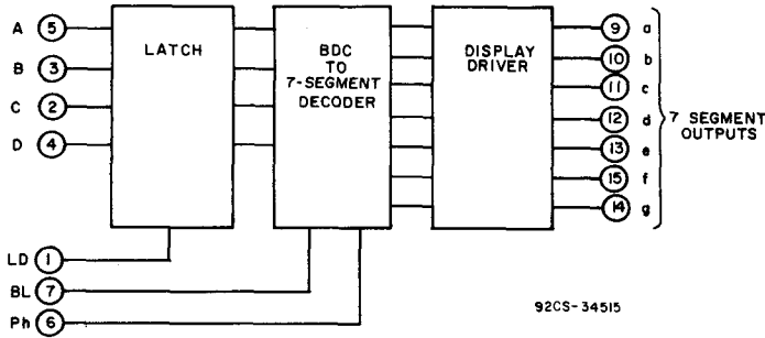
BCD-to-7-Segment Latch/Decoder/Driver
